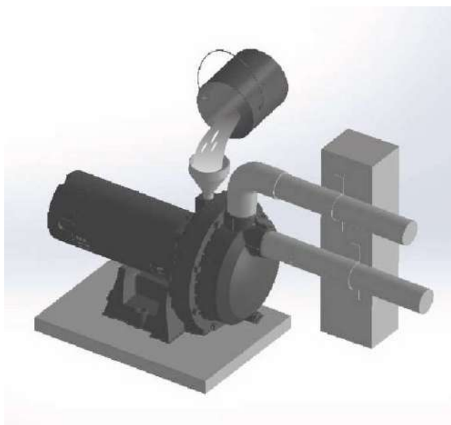
Figure 5: Fill Pump Before Starting
