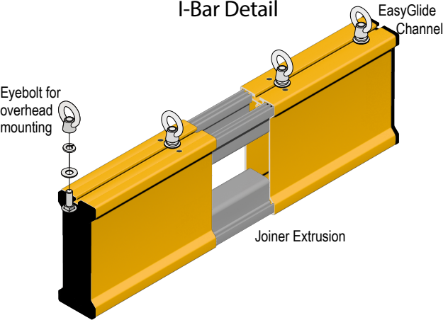
I-Bar Detail
