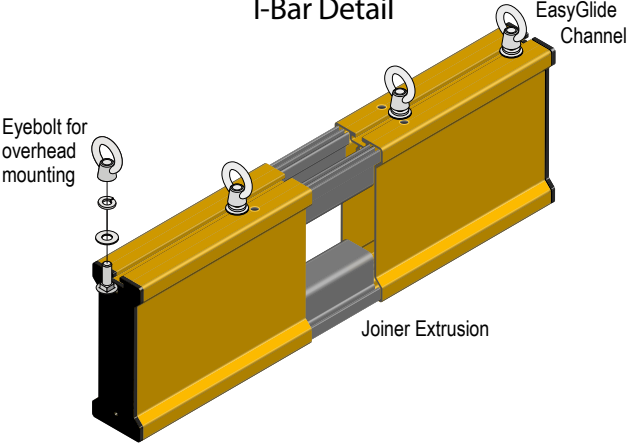
I-Bar Detail
